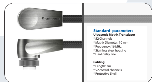
Ultrasonic Transducer
